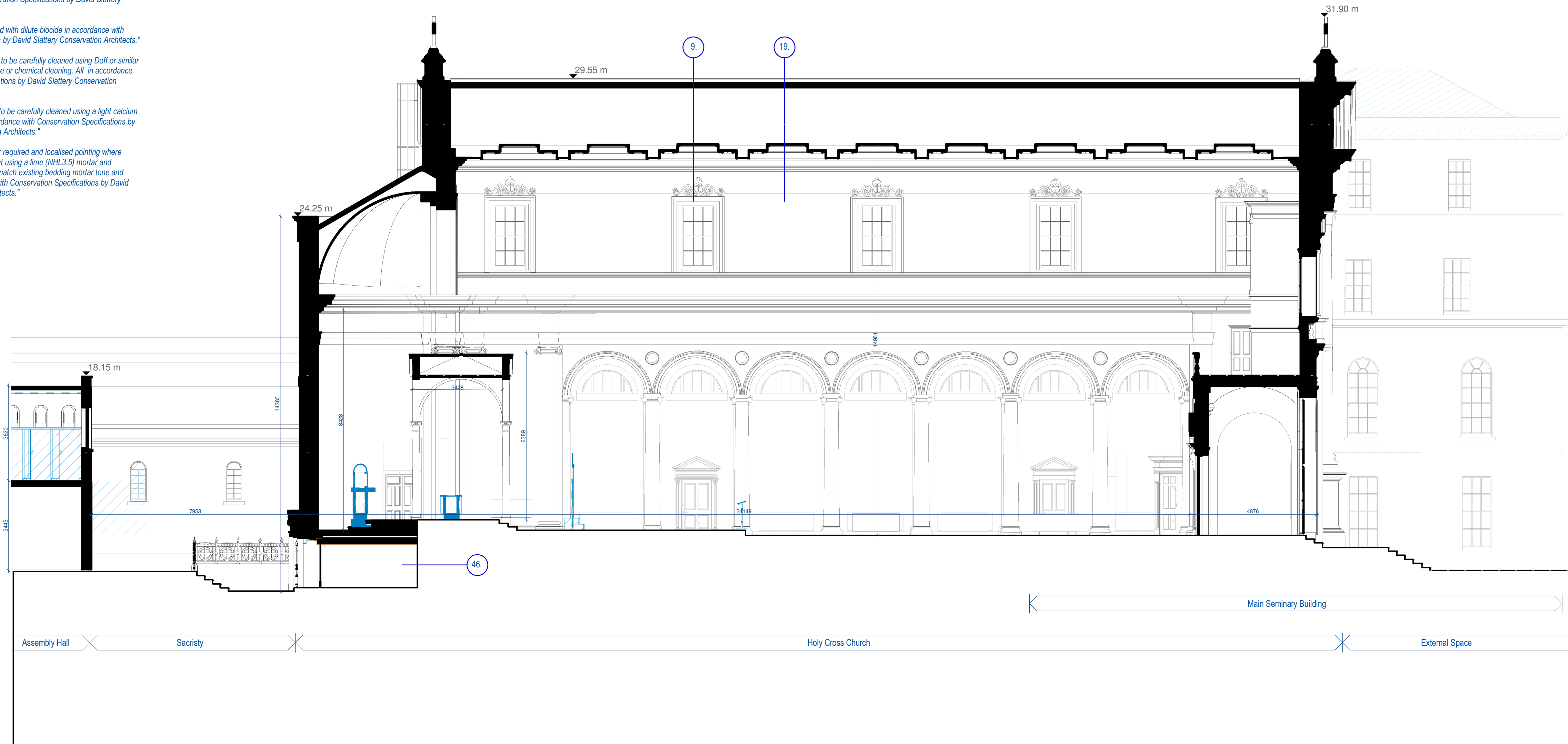
1 Church - Demolition Section AA Scale - 1:100
